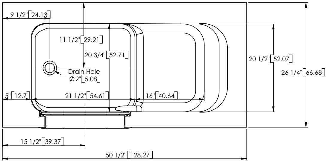
TOP VIEW
