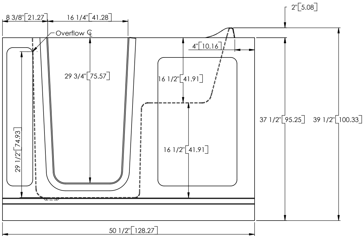
FRONT VIEW
