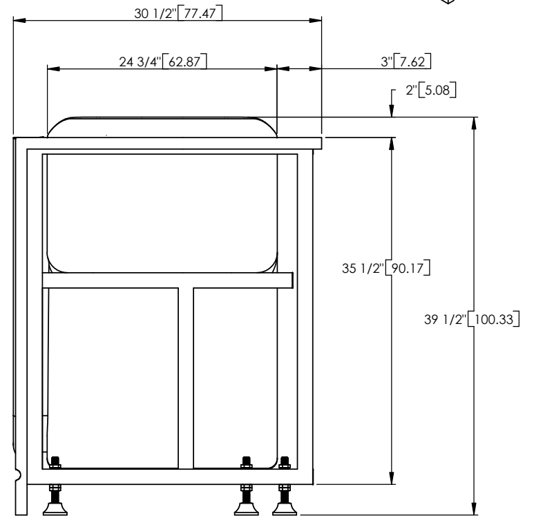
SIDE VIEW
